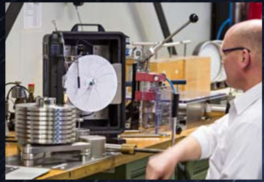
PRESSURE CALIBRATION 0-4000 bar (60.000 psi)
